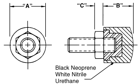
Molded Round Bumpers with Male Thread and Hex Shoulder EMRB 516 SERIES
