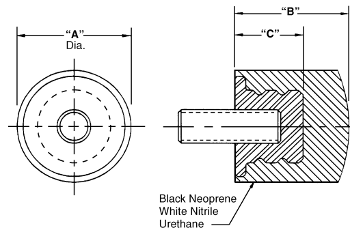
Molded Round Bumpers with Male Thread
