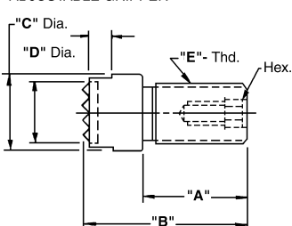
ADJUSTABLE GRIPPER
