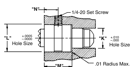
MOUNTING
