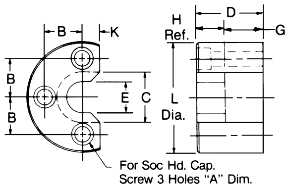
Screw Mount
