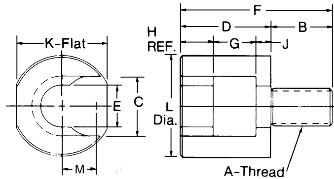
Male Thread Mount
